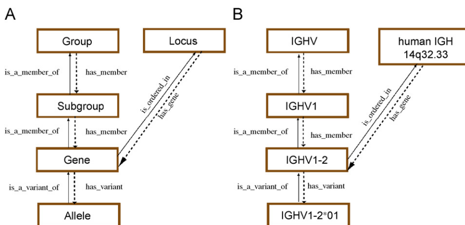
Figure 2 Concepts of classification for gene and allele nomenclature (CLASSIFICATION axiom). (A) Hierarchy of the concepts of classification and their relations. (B) Examples of concept instances for each concept of classification. The concept instances are associated with an instance of the "Taxon" concept, and more precisely for the "Gene" and "Allele" concepts with an instance of the "Species" concept (here, Homo sapiens ). The "Locus" concept is a concept of localization (LOCALIZATION axiom).
